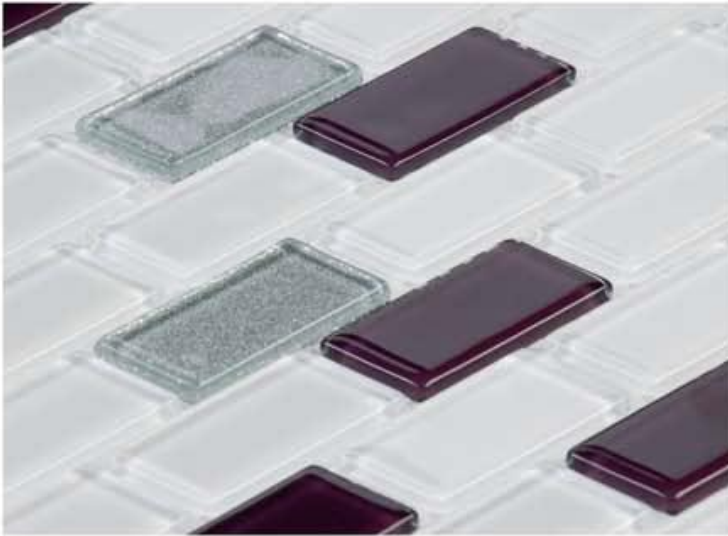
MP456 23x48x4 mm
